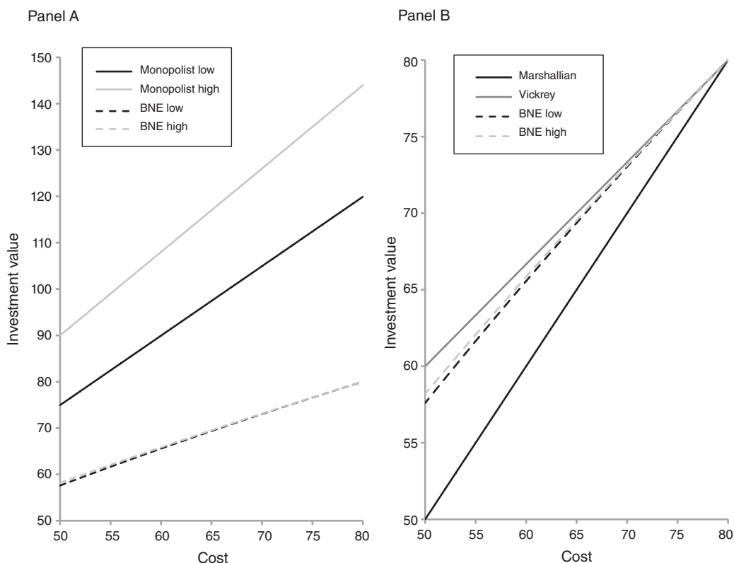
FIGURE 1. BNE THRESHOLD VALUES FOR TRIOPOLIES WITH COSTS DRAWN INDEPENDENTLY FROM THE UNIFORM DISTRIBUTION ON [50, 80]
