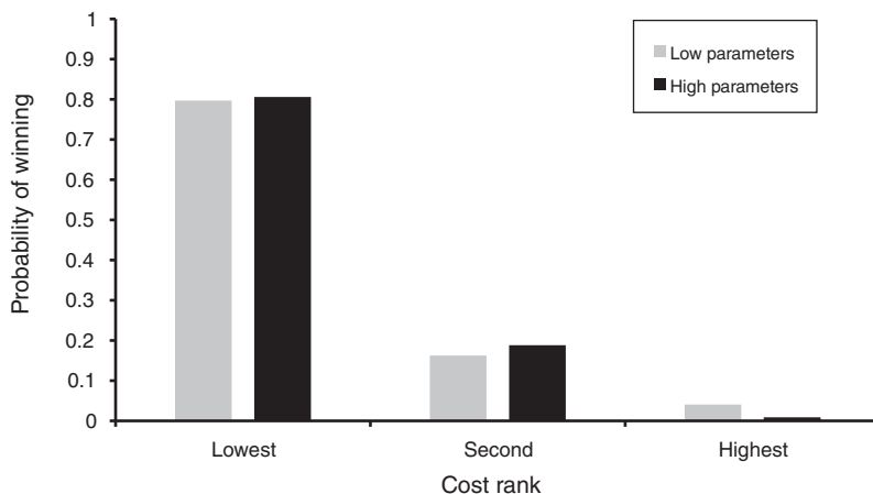
FIGURE 5. PROBABILITY OF PREEMPTING BOTH RIVALS AS A FUNCTION OF COST RANK
